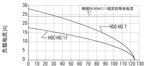
HDC-HQ7 and HDC-HQ17 / H07V-K2.5
