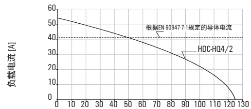
HDC-HQ4/2 / H07V-K6.0
