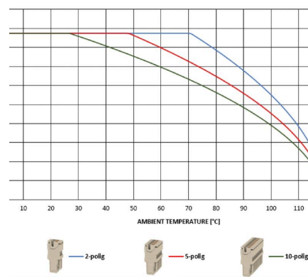
Derating APG 1.5...
