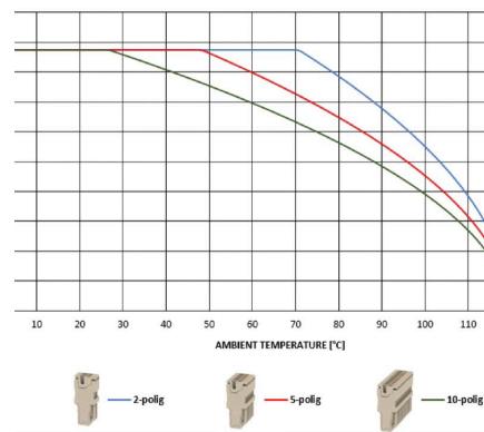
Derating APG 1.5...
